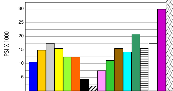
COMPRESSIVE STRENGTH
